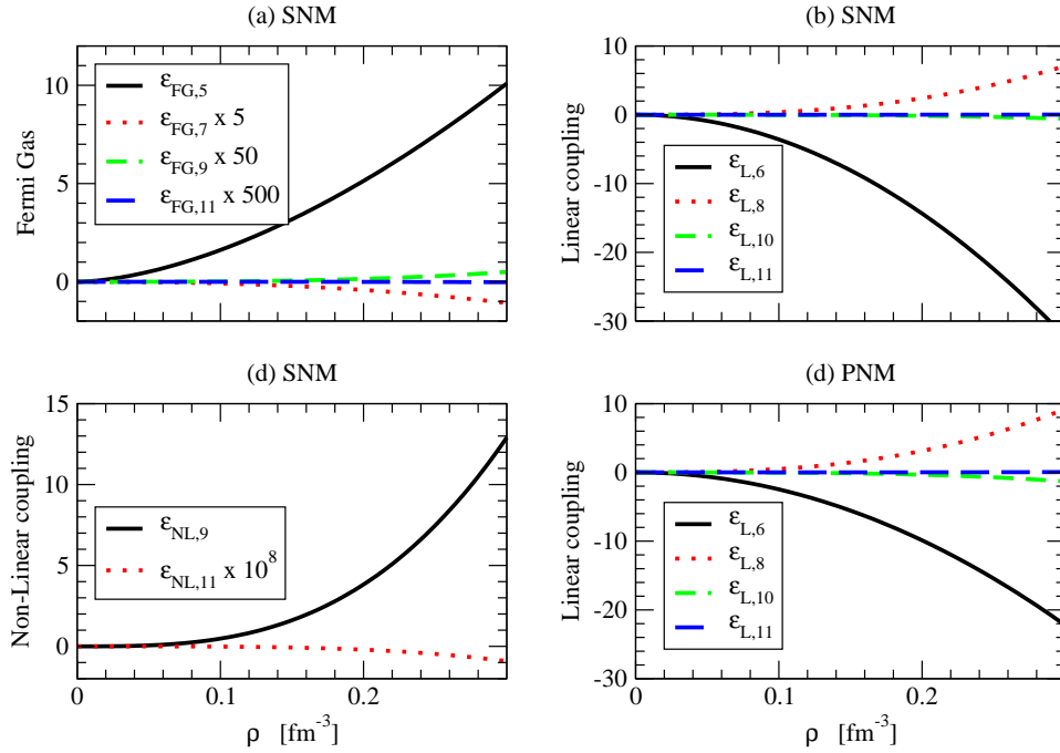
FIG. 2: (Color online) Representation of the different terms in the serie expansion of the energy functional with respect to the baryonic density, up to 0.3 \text{ fm}^{-3} . The first 3 subsets show the fast convergence in symmetric nuclear matter (SNM) and the last subset (d) show the contribution of the isovector mesons in pure neutron matter (PNM). To give an idea of the fast convergence, we have multiplied some of the terms by huge constants. The coupling constants (set A NL\rho\delta ) obtained by Liu et al. [42] has been used.
