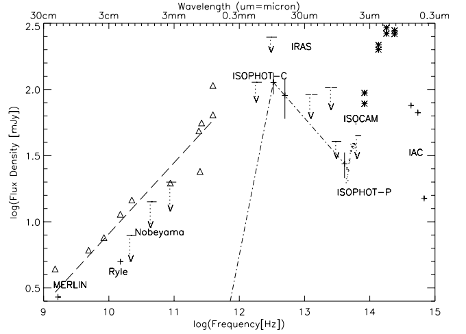
Fig. 6. Same as Fig. 3, with, in addition: the synchrotron spectrum of a power-law distribution fitting the infrared data (dash-dot lines of indices 2.5 and the measured value of \leq -0.6 ), and the line fitting the radio-to-submillimetre average fluxes (large dashed line of index 0.5).
