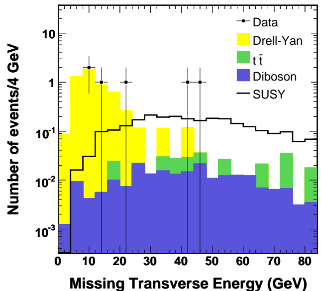
Figure 1: Missing transverse energy distribution for the ee\tau analysis after all the selection criteria are applied except for the cut \cancel{E}_T > 20 GeV. The observed data (points) are compared to the sum of the SM contributions (stacked, filled histograms). The open histogram shows the expected SUSY contribution for the mSUGRA scenario described in the text with m_{\tilde{\chi}_1^\pm} = 113 GeV/ c^2 and \sigma \times \mathcal{B} = 0.6 pb.
