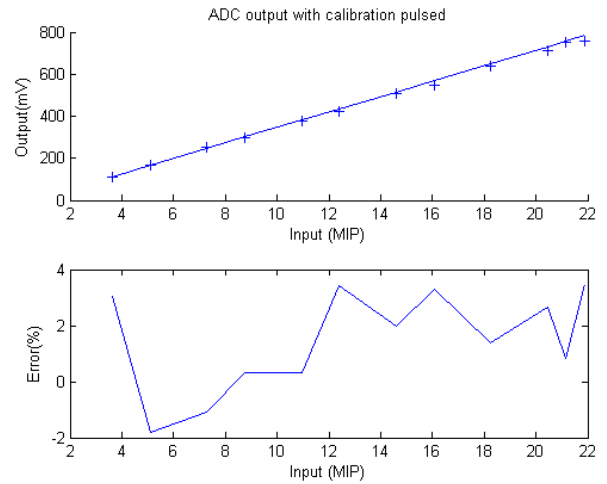
Figure 8: Digitized calibration pulses responses for a 1-22 MIP input range
