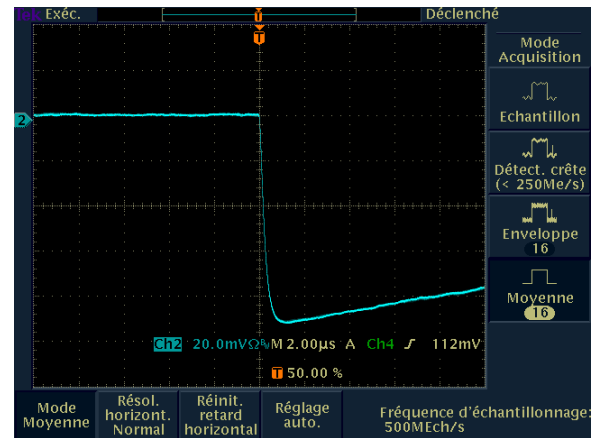
Figure 3: Preamplifier output
