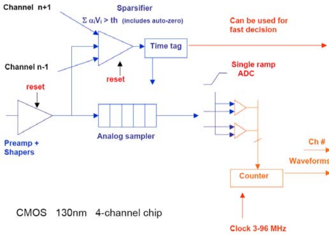
Figure 1: Foreseen front-end chip architecture
