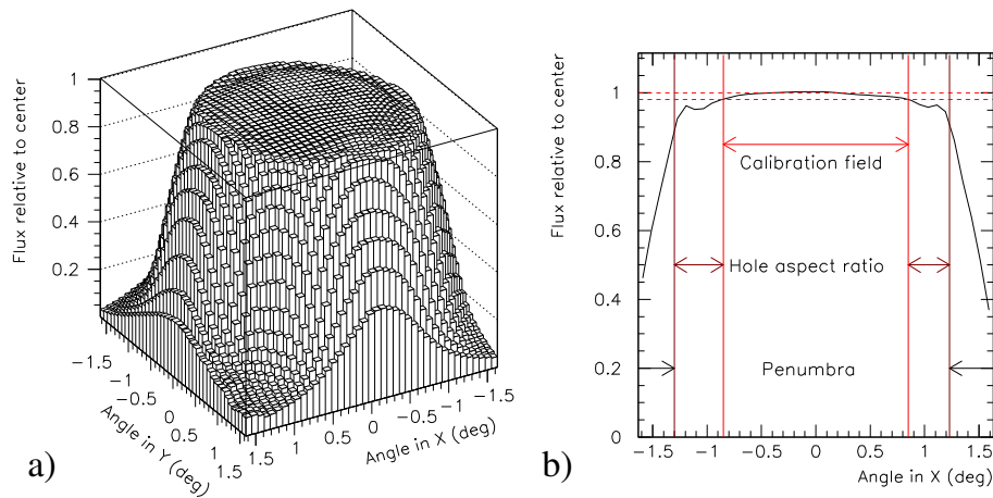
Figure 5: a.)XY scan of the illumination field of the LED light source in Figure 4. The photocurrent measured in the central flat field, generated by a 5.8 mm 2 photodiode at 0.9 m, is about 12 pA. b.) A cut of this field along a symmetry axis shows a \pm 0.8^\circ calibration field with a \pm 1\% uniformity, surrounded by a rougher region of 0.4^\circ due to a bad aspect of the angular diaphragm and a penumbra zone.
