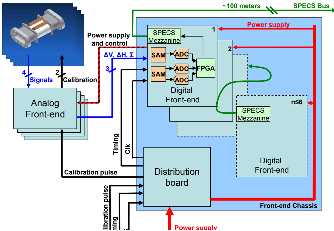
Figure 2 Hardware configuration
