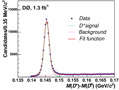
FIG. 1: The mass difference M(D^*) - M(D^0) for events with 1.8 < M(D^0) < 1.95 GeV/c 2 and an associated muon. The number N_{D^*\mu} was defined as the number of signal events in the mass difference range of 0.142–0.149 GeV/c 2 .
