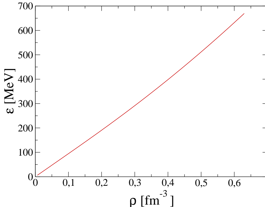
FIG. 6: Energy density versus baryonic density for cold uniform matter in beta equilibrium. The calculation is done in the scheme corresponding to the last column of Table 1.
