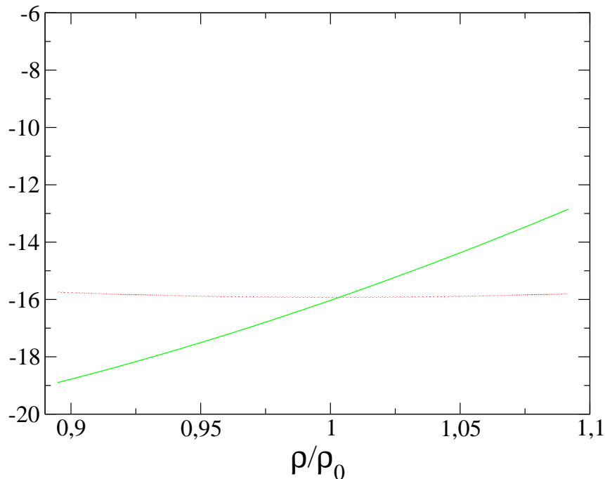
FIG. 3: Chemical potential with (solid line) or without (dashed line) inclusion of the rearrangement terms. For comparison, the energy per particle (dotted line) is also shown.
