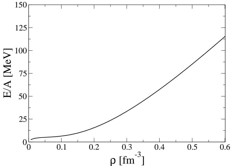
FIG. 6: Energy per particle versus baryonic density for cold uniform matter in beta equilibrium. The calculation is done in the scheme corresponding to the last column of Table 1.
