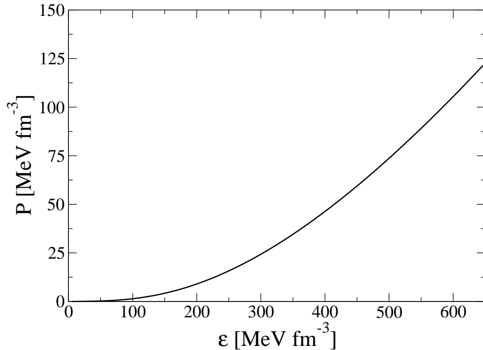
FIG. 7: Equation of state of cold uniform matter in beta equilibrium : pression versus energy density. The calculation is done in the scheme corresponding to the last column of Table 1.
