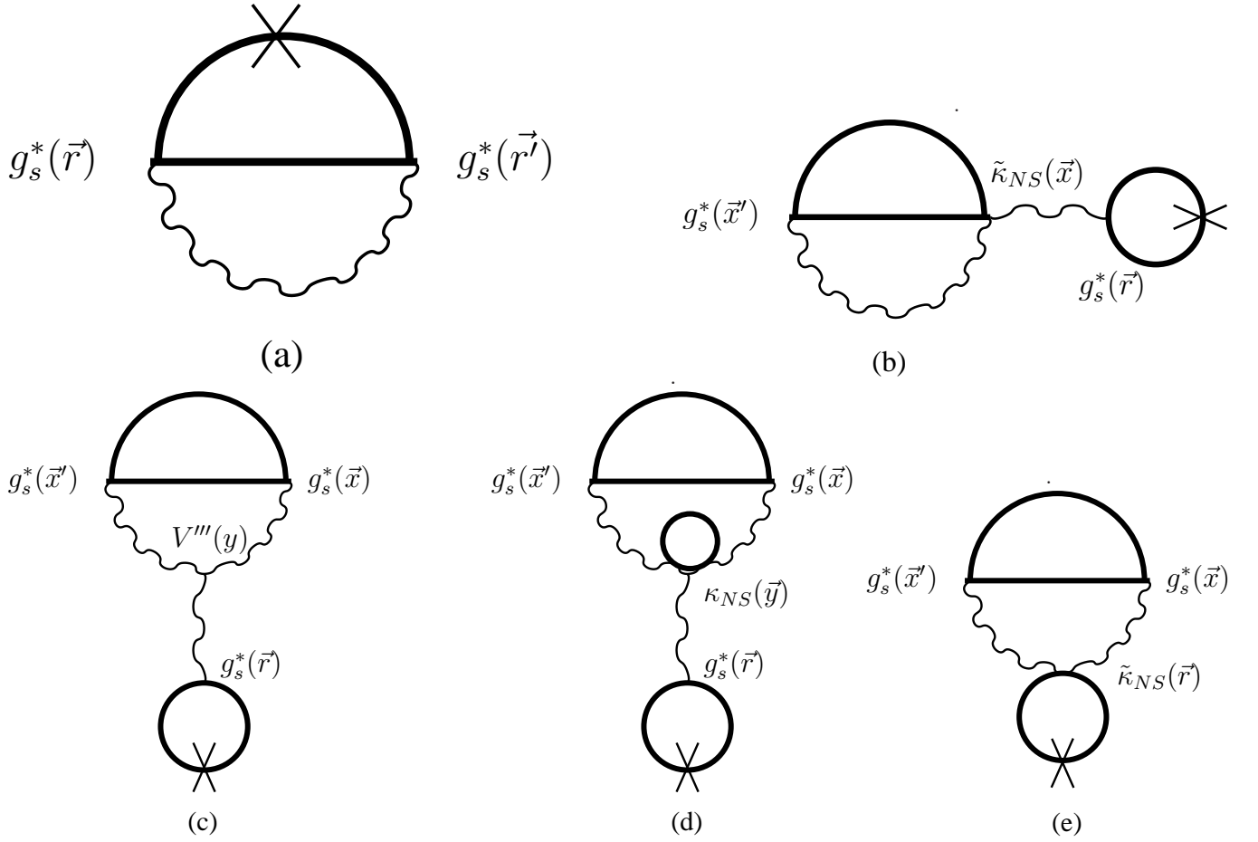
FIG. 1: Rearrangement terms; the crosses indicate the opening of a line to generate the various contributions to the single-particle hamiltonian. Detailed explanations are given in the text.
