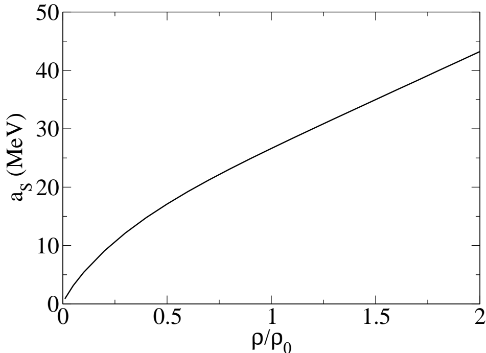
FIG. 4: Asymmetry energy versus density. The calculation is done with the inclusion of the contact terms and when the scalar polarizability \tilde{\kappa}_{NS} depends on \bar{s} .
