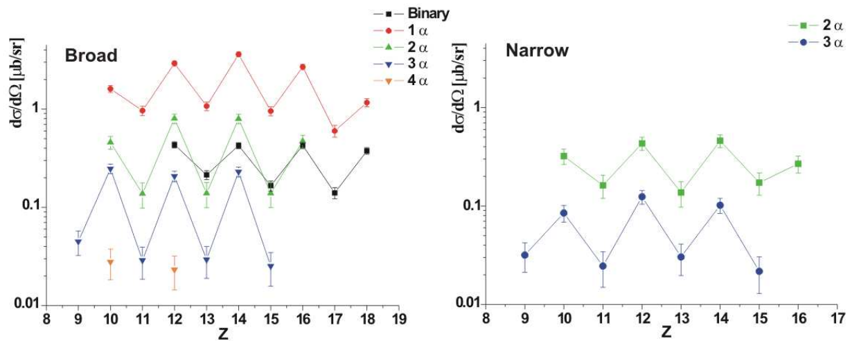
FIG. 20: (Color online) Differential cross sections in the reaction ^{36}\text{Ar} + ^{24}\text{Mg} for channels defined by (Z_3+Z_4+x\alpha) of the broad (binary) and narrow (ternary) components of the coincident fission fragments. They represent the average over the angular range between \theta_{c.m.} = 65^\circ to 120^\circ in the centre-of-mass system. The fission channels with missing 1\alpha , 2\alpha , 3\alpha and 4\alpha -particles are shown.
