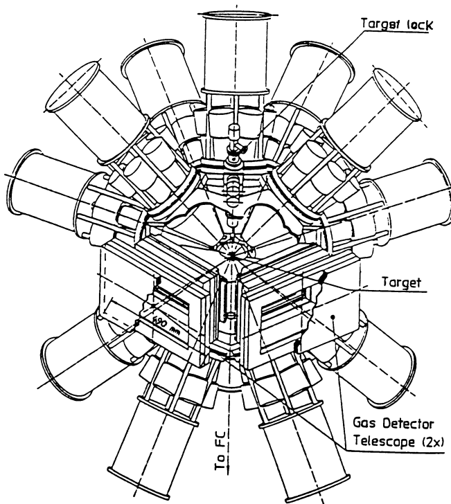
FIG. 1: The BRS-OSIRIS set-up used for the study of coincident fission channels in the reactions ^{36}\text{Ar} + ^{24}\text{Mg} \rightarrow Z_3 + Z_4 + \Delta Z , at E_{lab}(^{36}\text{Ar}) = 195 MeV. The OSIRIS \gamma -detector array consisted of 12 Compton-suppressed Ge-detectors.
