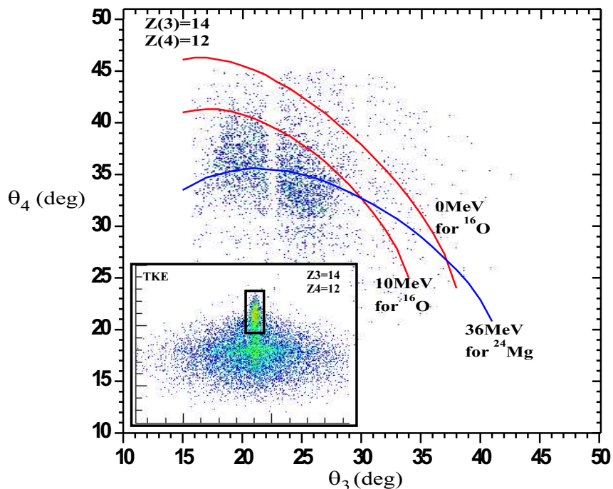
FIG. 16: (Color online) In-plane \theta_4 vs. \theta_3 (in degrees) correlations, of coincident fragments for the channels gated on the narrow (ternary) components for definite values Z_3+Z_4 for the fission defined by Z_3+Z_4+2\alpha . The kinematical calculations are shown for the Mg-target and for the O-target (channel Z_3+Z_4+0\alpha representing a binary channel) with the effective Q-values as indicated and as discussed in the text. The angular range in the centre of mass frame is between \theta_{c.m.}=65^\circ to 120^\circ .
