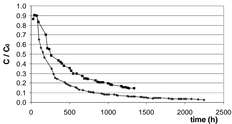
Fig 9: Silicic acid desorption by flushing the compacted magnetite column with 0.01M NaCl. Results are given for columns loaded in the initial sorption experiment with an inlet stock solution for the adsorption of H_4SiO_4 of (■) 4.5 \times 10^{-4} M ; (◇) 1.6 \times 10^{-3} M .
