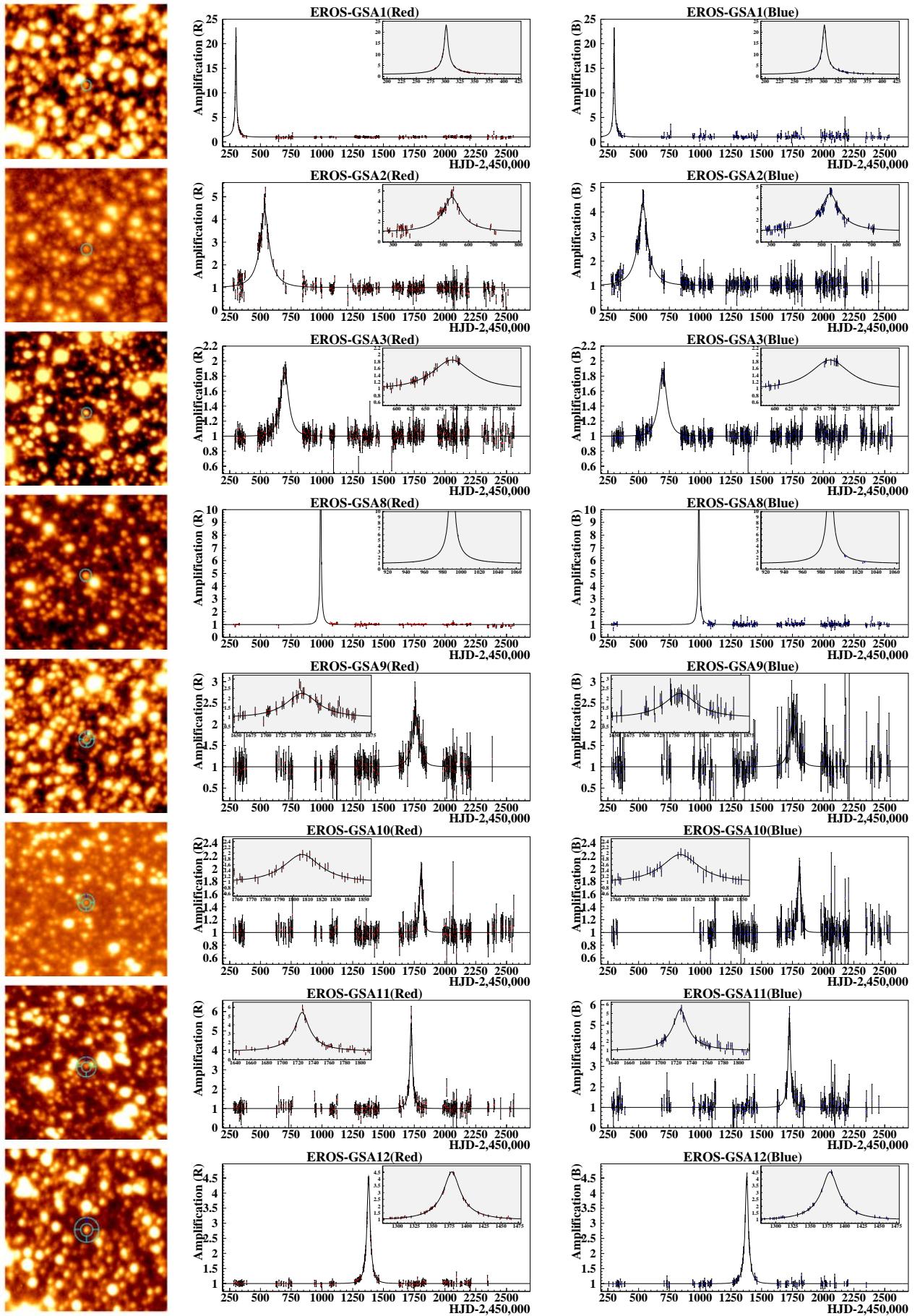
Fig. 22. Finding charts (84"×84", N-up, E-left) and magnification of the candidates as a function of the Heliocentric Julian Day ( HJD-2,450,000 ). In the case of multi-detected events, we display only the best sampled light curve.
