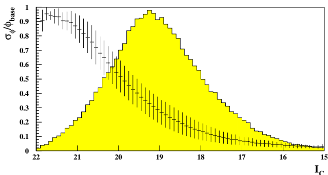
Fig. 6. Average photometric point-to-point precision along the light-curves versus I_C . The vertical bars show the dispersion of this precision in our source sample. The histogram shows the magnitude distribution of the full catalog (average over 4 directions).
