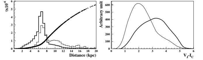
Fig. 11. Left: Optical depth as a function of the distance (thick line), source distance distribution of a simulated catalog (thick histogram), and distance distribution weighted by the optical depth (thin histogram). Right: color distribution of the stars of the simulated catalog (thin line) and expected color distribution of the lensed stars (thick line).
