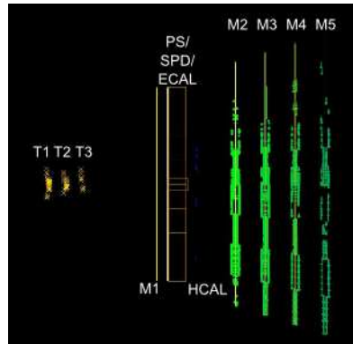
Figure 2. First beam particles through the LHCb subdetectors lying after the magnet (M1 & ECAL were not read out for this event).
