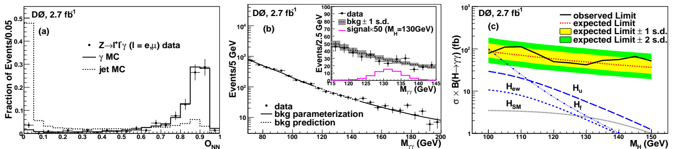
FIG. 1: (color online). (a) Normalized O_{NN} spectrum for photons and jets. (b) M_{\gamma\gamma} spectrum in data (points) compared to the total background parameterization (solid line), including the DDP contribution derived via a sideband fit, and the total background prediction (dashed line) inside the search region for M_H = 130 GeV. The inset figure compares the data to the total background prediction inside the search region including its one standard deviation (s.d.) uncertainty band, as well as the expected H_{SM} signal scaled by a factor of 50. (c) Observed and expected 95% C.L. upper limits on \sigma \times B as a function of M_H . Also shown are the predictions for \sigma \times B in the different EWSB scenarios discussed in the text.
