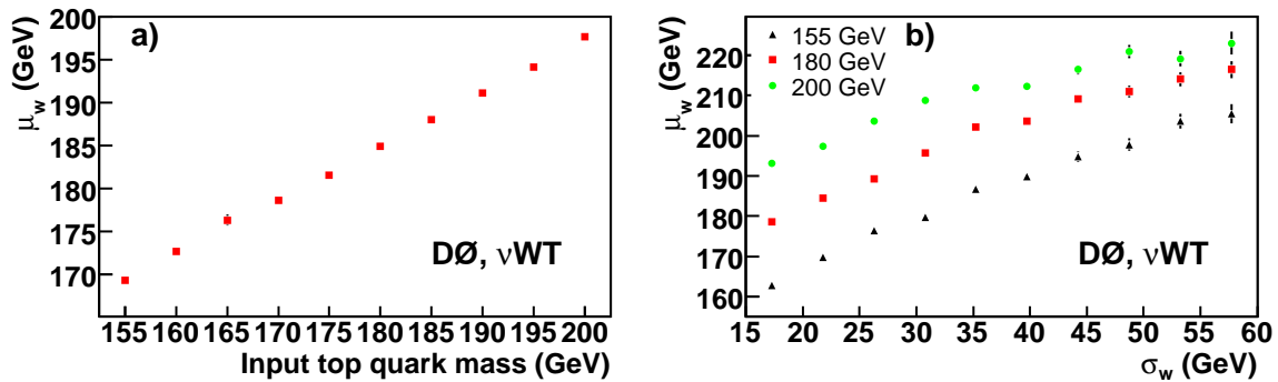
FIG. 5: (a) Correlation between the mean of the \nu WT weight distribution and the input m_t . (b) Correlation between \nu WT \mu_w and \sigma_w for the e\mu channel. Three test masses of 155 GeV, 180 GeV, and 200 GeV are shown.
