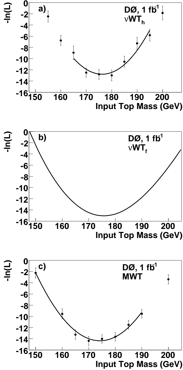
FIG. 11: Negative log-likelihood -\ln \mathcal{L} vs. m_t for the combination of all channels before calibration for the (a) \nu\text{WT}_h , (b) \nu\text{WT}_f , and (c) MWT methods.
