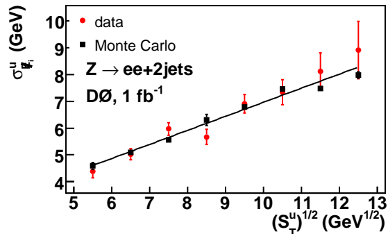
FIG. 3: Dependence of the resolution of unclustered E_T on the unclustered scalar transverse missing energy for Z \rightarrow ee events with exactly two jets.
