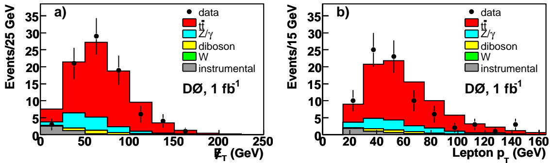
FIG. 2: (a) \cancel{E}_T and (b) leading lepton p_T for t\bar{t} ( m_t = 170 GeV) and background processes overlaid with those for observed events in all channels after final event selection. We assume \sigma_{t\bar{t}} = 7.0 pb.
