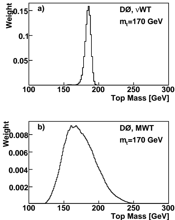
FIG. 4: Example weight distributions for different single t\bar{t} \rightarrow e\mu Monte Carlo events obtained with a) \nu WT method and b) MWT method. The generator level mass is m_t = 170 GeV.
