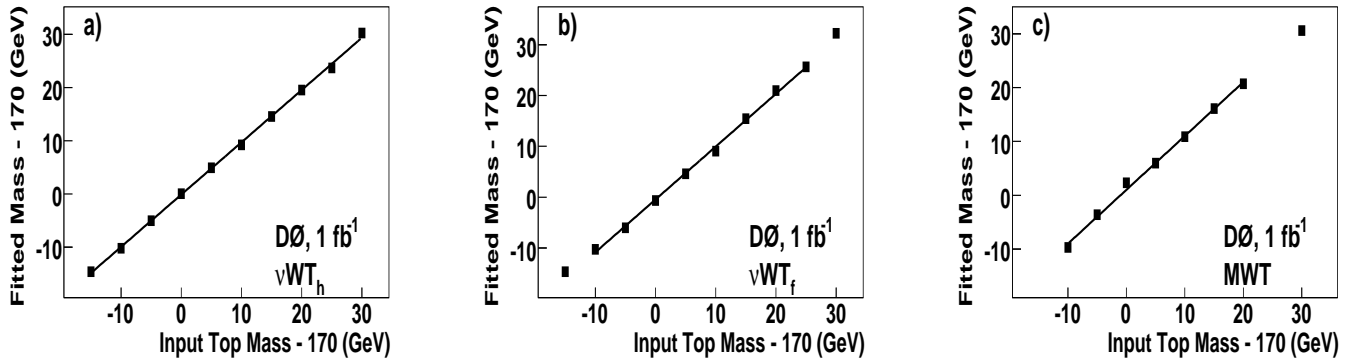
FIG. 9: The combined calibration curves corresponding to the (a) \nu\text{WT}_h , (b) \nu\text{WT}_f , and (c) MWT methods. Overlaid is the result of the linear fit as defined in Eq. 20. The uncertainties are small and corresponding bars are hidden by the markers.
