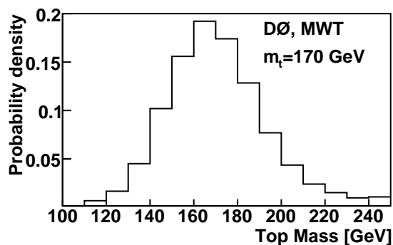
FIG. 6: An example of a template for the MWT method.
