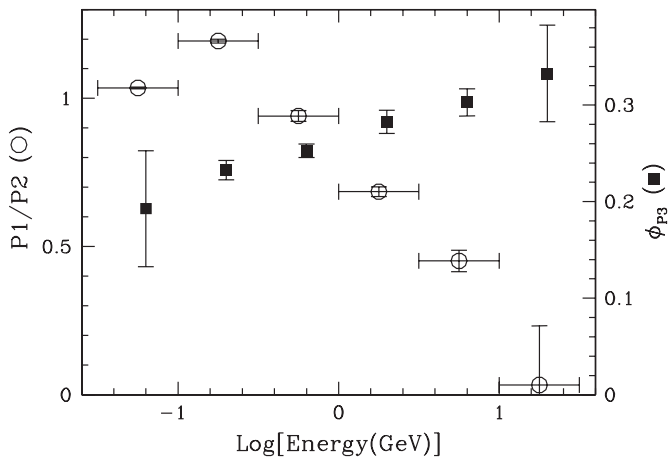
Figure 3. Evolution of the P1/P2 pulse peak ratio (open circles) and the P3 pulse peak phase (solid squares) with energy.
