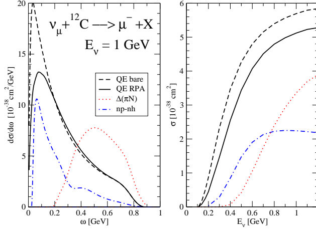
FIGURE 2. Left panel: differential \nu_\mu - ^{12}\text{C} charged current cross-section as a function of transferred energy in the various channels for E_\nu=1 GeV. Right panel: total \nu_\mu - ^{12}\text{C} charged current cross-section in the various channels.
