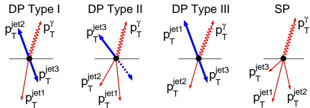
FIG. 2: Diagrams of DP Types I, II, III and SP \gamma + 3 jets events. For DP events, the light and bold lines correspond to two separate parton interactions. The dotted line represents unreconstructed jet.
