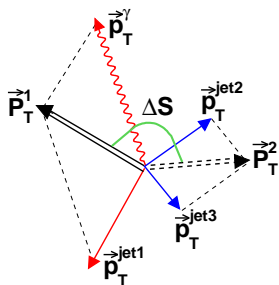
FIG. 5: A possible orientation of photon and jets transverse momenta vectors in \gamma + 3 jets events. Vectors \vec{P}_T^1 and \vec{P}_T^2 are the p_T imbalance vectors of \gamma +jet and jet-jet pairs. The figure illustrates a general case for the production of \gamma + 3 jets +X events.
