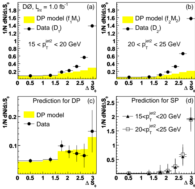
FIG. 7: Results of the two datasets fit for the \Delta S_\phi variable for the combination of two p_T^{\text{jet}2} bins 15 – 20 GeV and 20 – 25 GeV. (a) and (b) show distributions for data (points) and the DP model (shaded area); (c) shows the prediction for DP from data (points), corrected to remove SP contribution, and the DP model (shaded area) as a difference between the corresponding distributions of (a) and (b); (d) shows the extracted SP distributions in the two bins. The error bars in (a) and (b) are only statistical, while in (c) and (d) they represent total (statistic and systematic) uncertainty.
