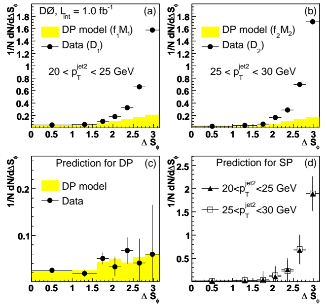
FIG. 8: Same as in Fig. 7 but for the other combination of p_T^{\text{jet}2} bins, 20 – 25 GeV and 25 – 30 GeV.
