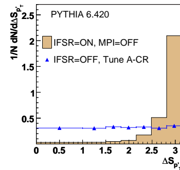
FIG. 9: \Delta S_{p_T} distributions for \gamma + 3 jets events simulated using PYTHIA with ISR/FSR but with MPI switched off (shaded region), as well as for \gamma + 3 jets events without ISR/FSR but MPI switched on using Tune A-CR (triangle markers). The bin 15 < p_T^{\text{jet}2} < 20 GeV is considered.
