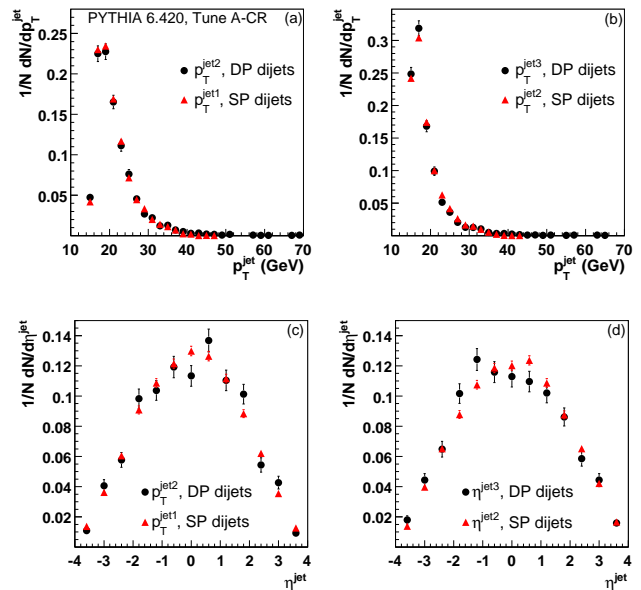
FIG. 12: Comparison of dijet events properties in SP (triangles) and in \gamma + 3 jets DP events (black circles): (a) and (c) show comparisons of the p_T and \eta distribution of the second (ordered in p_T ) jet in \gamma + 3 jets DP events with the first jet from the SP dijet events; (b) and (d) show comparisons of the p_T and \eta distribution of the third jet in \gamma + 3 jets DP events with the second jet from the SP dijet events. Both types of events are generated without ISR and FSR effects but with MPI Tune A-CR.
