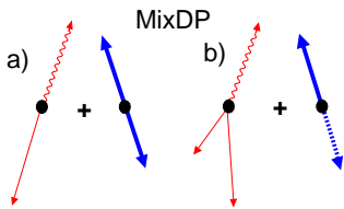
FIG. 4: Description of the mixing procedure used to prepare the MixDP signal sample. Two combinations of mixing \gamma + 1 jet and two jets from dijet events (a) and \gamma + 2 jets and one jet from dijet events (b) are considered. The dotted line represents a jet failing the selection requirements.
