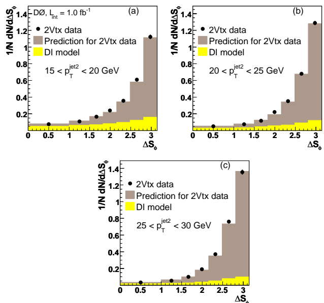
FIG. 10: \Delta S_\phi distributions for two-vertex \gamma + 3 jets events in the three p_T^{\text{jet2}} intervals: (a) 15 – 20 GeV, (b) 20 – 25 GeV and (c) 25 – 30 GeV. MixDI and the total sum of the MixDI and Bkg2Vtx distributions (shaded histograms) are weighted with their fractions found from the fit, compared to 2Vtx data (black points). The shown uncertainties are only statistical.
