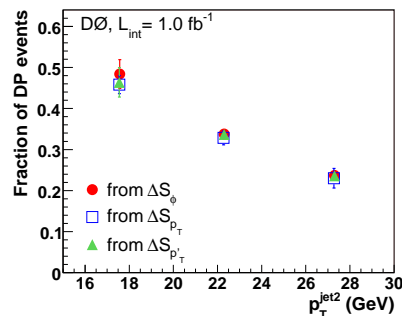
FIG. 6: Fractions of DP events extracted with the \Delta S_\phi , \Delta S_{p_T} , and \Delta S_{p'_T} variables in the three p_T^{\text{jet}2} intervals.
