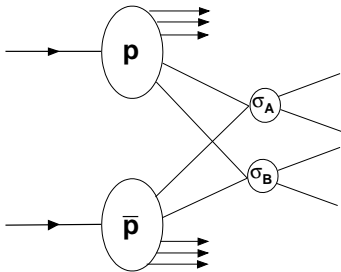
FIG. 1: Diagram of a double parton scattering event.
