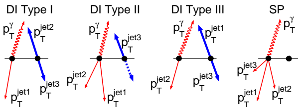
FIG. 3: Diagrams of DI Types I, II, III and SP \gamma + 3 jets events. For DI events, the light and bold lines correspond to two separate p\bar{p} interactions. The dotted line represents unreconstructed jet.
