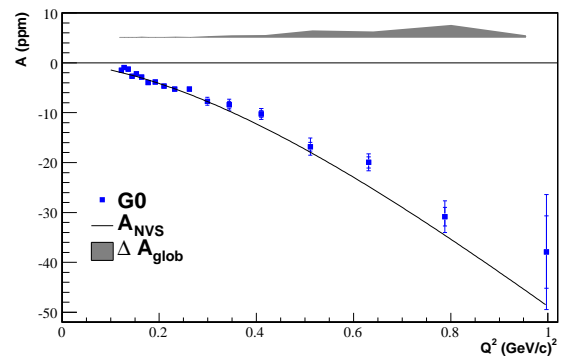
Fig. 12. Results of the forward angle experiment
