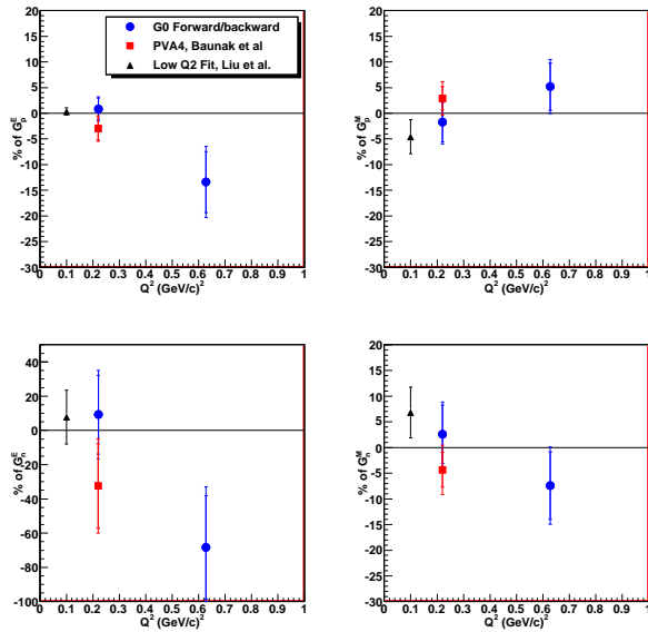
Fig. 19. Electric (left) and magnetic (right) contribution of the strange quarks to the electromagnetic form factors of the proton (above) and neutron (below) in percent
