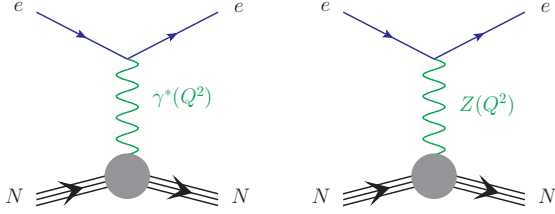
Fig. 1. Diagrams contributing to the elastic electron-nucleon scattering.
