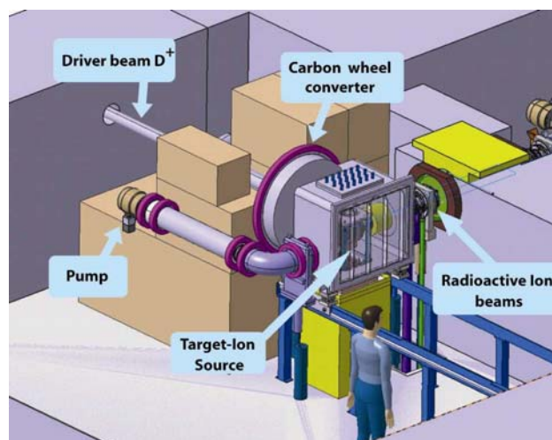
Figure 3: Spiral 2 UCx production module
