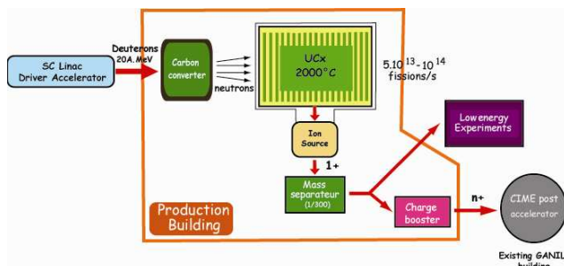
Figure 2 : RIB Production technique in Spiral 2
