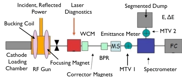
Figure 1: The PHIN photo-injector layout.
