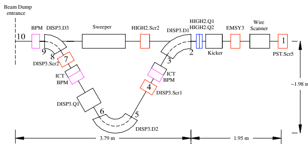
Figure 2: Layout of the foreseen HEDA2 setup.
