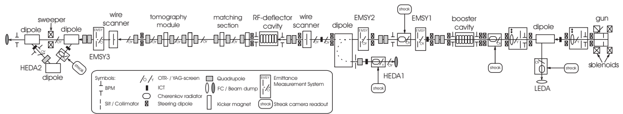
Figure 1: Layout of the future Photo Injector Test facility at DESY, Zeuthen site, (PITZ).
