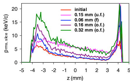
Figure 4: Simulated slice momentum spread compared to its reconstructed at the dispersive screen for different quadrupole focusing corresponding to the rms horizontal beam sizes at the reference screen. The abbreviations u.f., f, and o.f. present the under-focused, focused and over-focused conditions at the reference screen.
