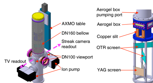
Figure 6: The first screen station in HEDA2 (DISP3.Scr1) including details of screens and slit configurations.
