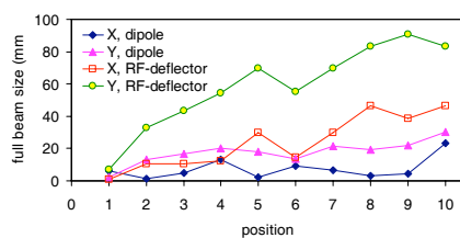
Figure 5: Calculated beam sizes along the HEDA2 section. The position numbers correspond to the numbers indicated in HEDA2 setup in Fig.2.
