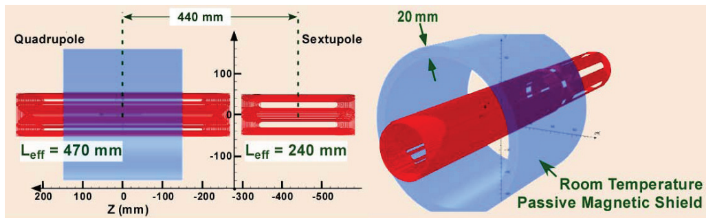
Figure 3: The ATF2 passive magnetic shield and coil layout. Effective magnetic lengths for the coils are as shown.
