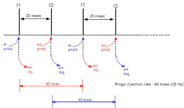
Figure 2: Timing process.
