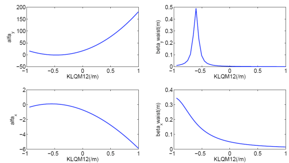
Figure 4: Strength change of QM12 influence on \alpha_x , \beta_x , \alpha_y and \beta_y .
