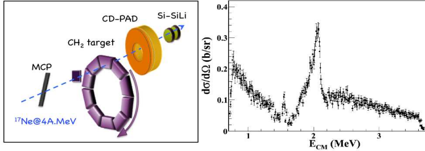
Fig. 1. Left: Experimental set-up for the study of ^{17}\text{Ne}(p, ^{17}\text{Ne})p resonant elastic scattering (see text for description). Right : Excitation function in the center -of-mass framework corrected from ^{12}\text{C} background and residual \beta p background from ^{17}\text{Ne} decay.
