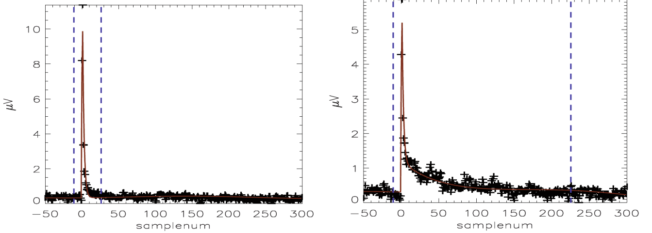
Fig. 9. Cosmic rays hitting the bolometers produce glitches with decay times depending on the part heated by the particle (after Tristram 2005).
