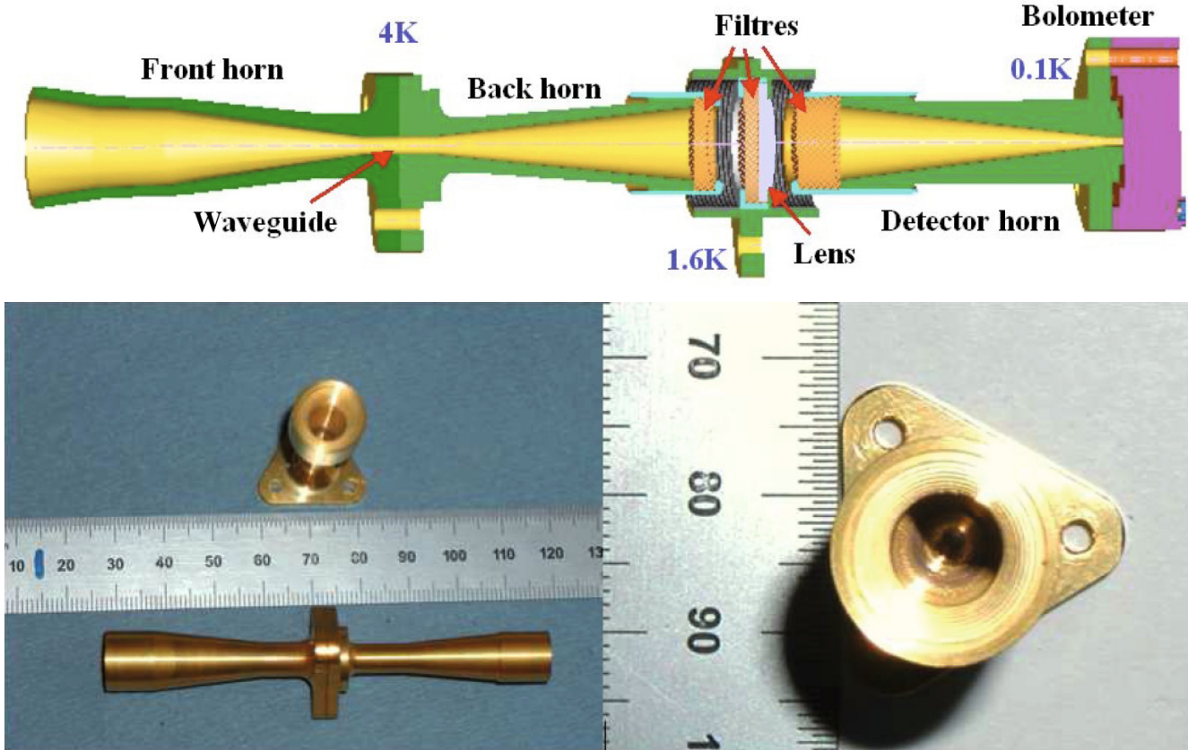
Fig. 1. A typical optical chain. The reference scale is in mm.
