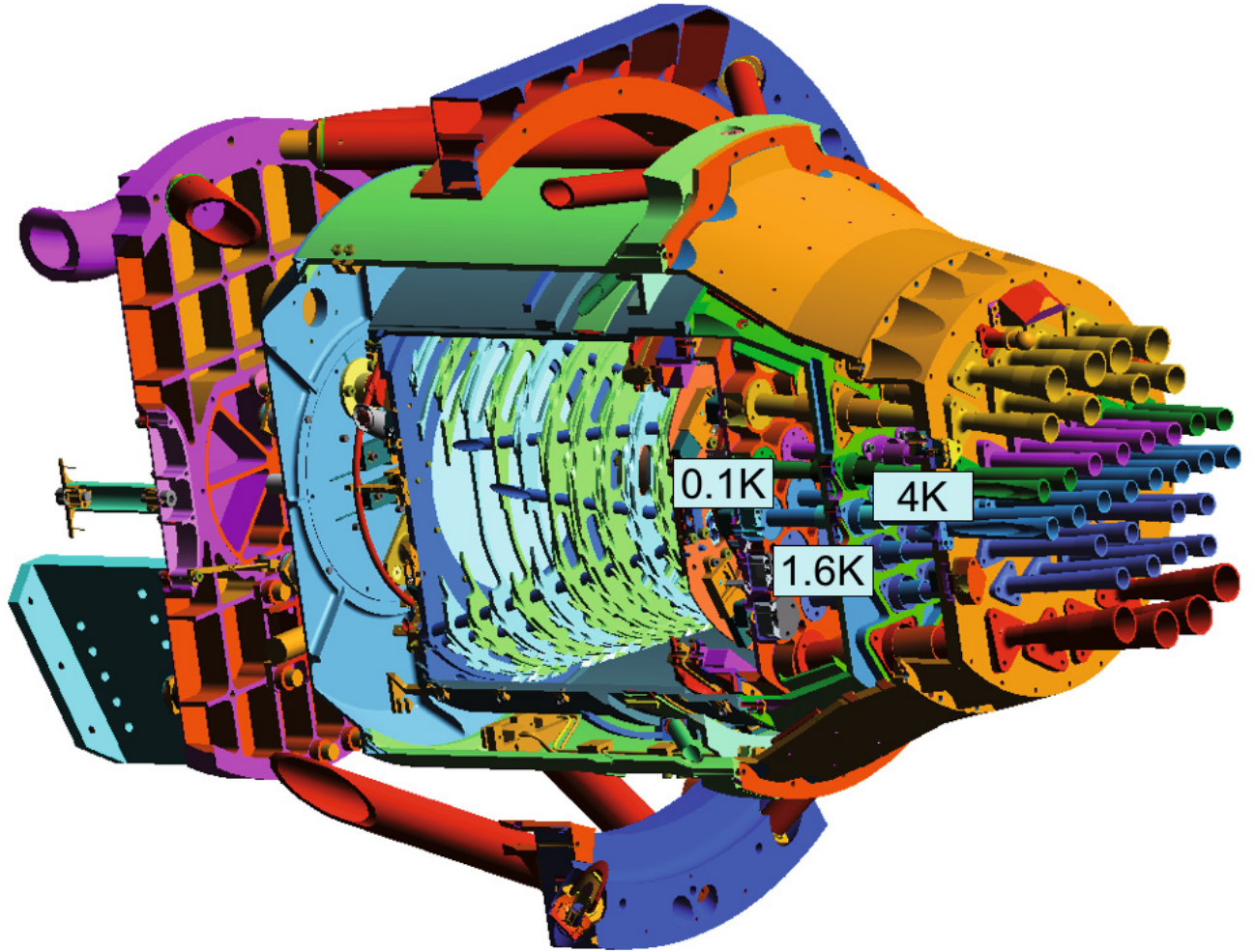
Fig. 2. The Russian doll arrangement of the HFI focal plane unit.
