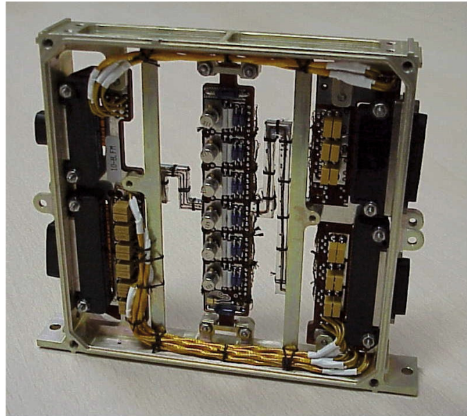
Fig. 15. Flight model of a six-channel JFETs board mounted on the 50 K stage. (Photo courtesy of Galileo Avionica.)
