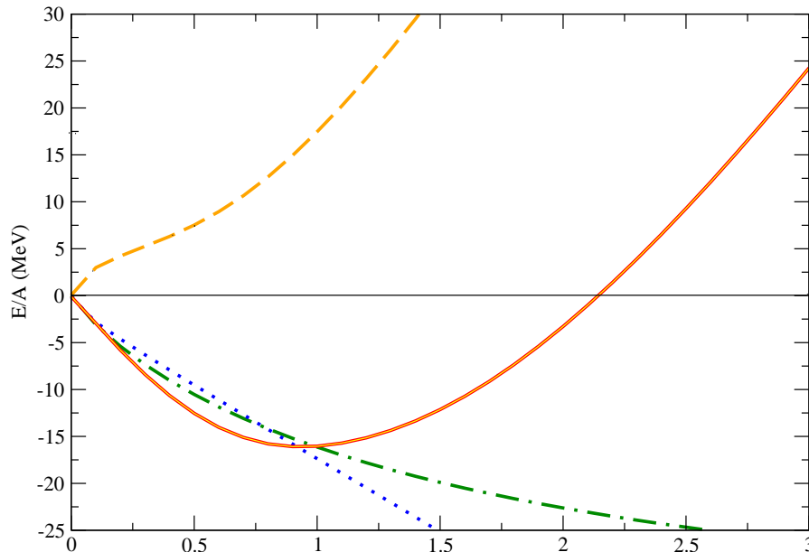
FIG. 2: Binding energy of nuclear matter versus nuclear matter density in units of normal density. The full line corresponds to the full result and the dashed line represents the Hartree result. The dot-dashed line corresponds to the contribution of the Fock term and the dotted line represents the correlation energy. All the numerical inputs are given in the text.
