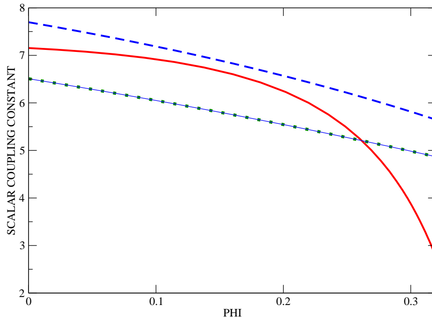
FIG. 3: effective scalar coupling constant versus the relative deviation, (M_0 - M)/M_0 \equiv |\bar{s}|/F_\pi , of the scalar field with respect to its vacuum value for the linear confining potential (dashed line), the quadratic linear potential (dotted line) and for the quark-diquark model (full line).
