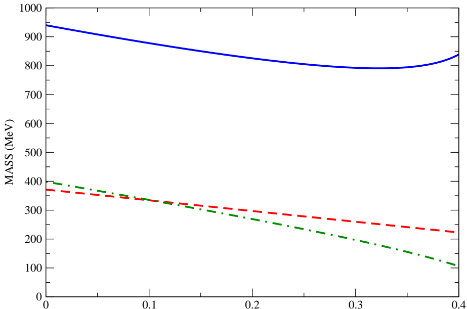
FIG. 1: Mass of the quark (dashed line), of the diquark (dot-dashed line) and of the nucleon (full line) versus the relative deviation, \Phi = (M_0 - M)/M_0 \equiv |\bar{s}|/F_\pi , of the scalar field with respect to its vacuum value.
