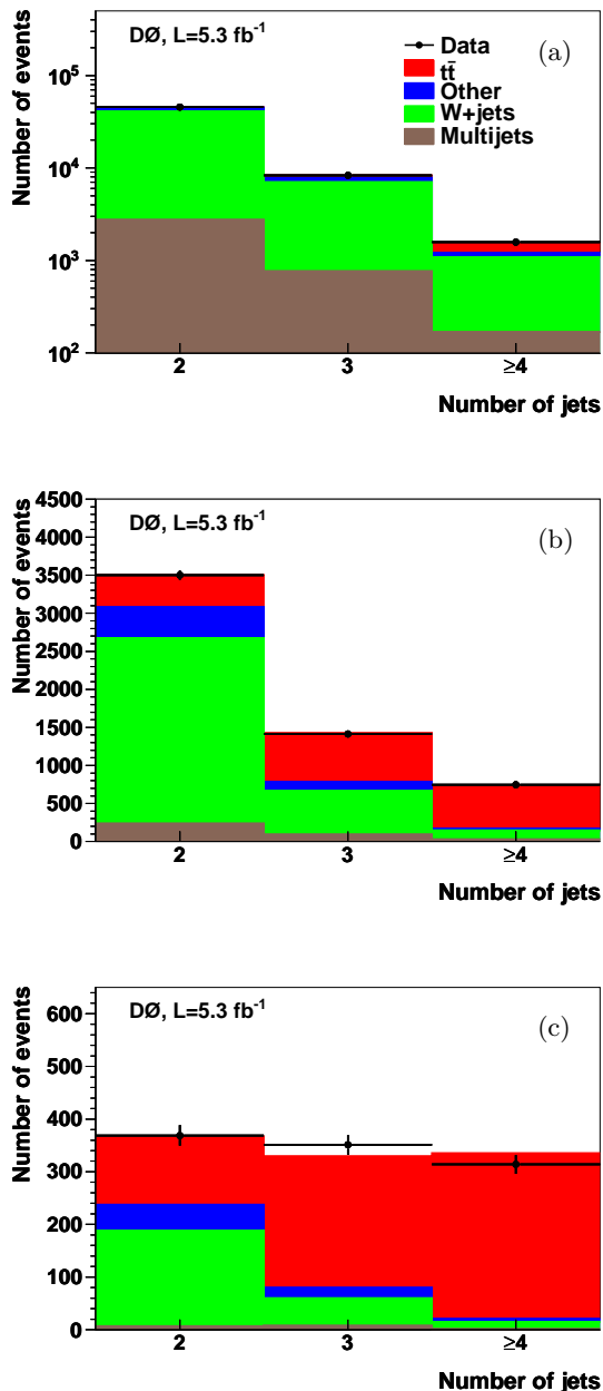
FIG. 5: (Color online) Jet multiplicity distributions for events with (a) 0, (b) 1, and (c) > 1 b -tagged jets for backgrounds and contributions from t\bar{t} signal for a cross section of 7.78 \text{ pb} as measured with the combined method.
