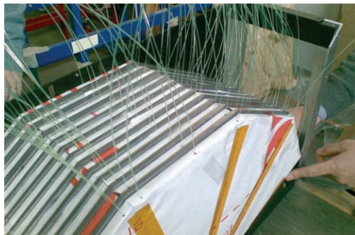
Figure 2: One of the four calorimeters modules during the assembly, wrapped tile, wavelength shifter, and lead plate are clearly visible.
