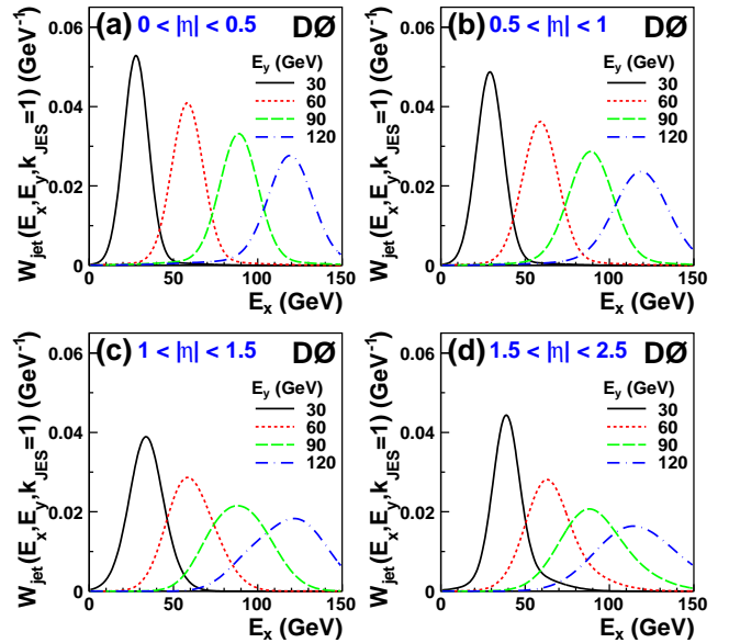
Figure 2. (color online) Transfer functions for k_{\text{JES}} = 1 light-quark jets as a function of measured jet energy for different parton energies in \eta regions: (a) |\eta| < 0.5 , (b) 0.5 < |\eta| < 1.0 , (c) 1.0 < |\eta| < 1.5 , and (d) 1.5 < |\eta| < 2.5 .
