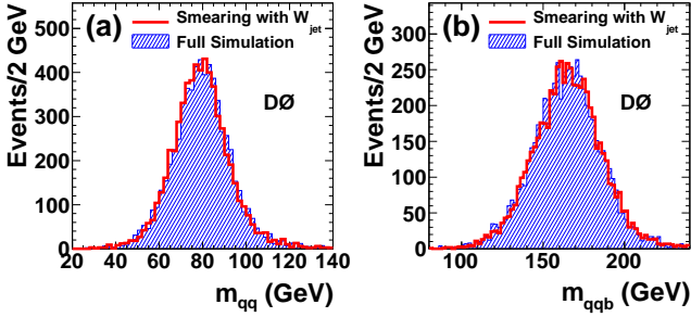
Figure 3. (color online) Comparison of (a) 2-jet and (b) 3-jet invariant mass distributions for parton-level t\bar{t} MC events with energies smeared using the transfer functions (open histogram) and fully simulated t\bar{t} MC events with all four jets spatially matched to partons (filled histogram).
