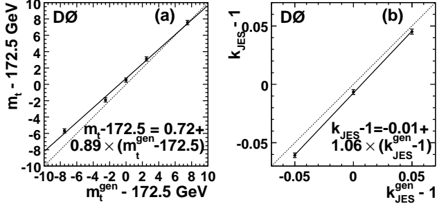
Figure 4. Mean values of (a) m_t and (b) k_{\text{JES}} extracted from ensemble studies, as a function of the input values fitted to straight lines. Dashed lines represent 1:1 correlations of extracted and input values.
