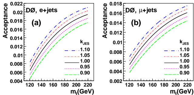
Figure 1. (color online) The mean acceptance as a function of m_t and k_{\text{JES}} for the (a) e +jets and (b) \mu +jets channels.
