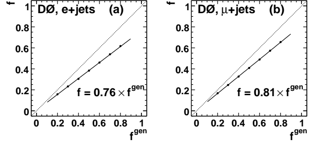
Figure 6. Extracted signal fractions from ensemble studies as a function of the input values for the (a) e +jets and (b) \mu +jets channels.
