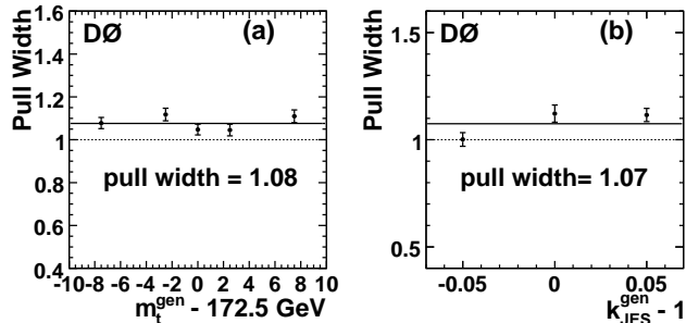
Figure 5. Widths of the pull distributions for (a) m_t and (b) k_{\text{JES}} from ensemble studies as a function of the input values.
