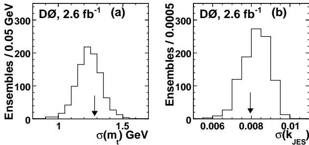
Figure 10. Expected uncertainty distributions for (a) m_t and (b) k_{\text{JES}} determined from 1000 pseudoexperiments performed on the MC t\bar{t} sample for m_t^{\text{gen}} = 175 GeV. The measured uncertainties are indicated by the arrows.
