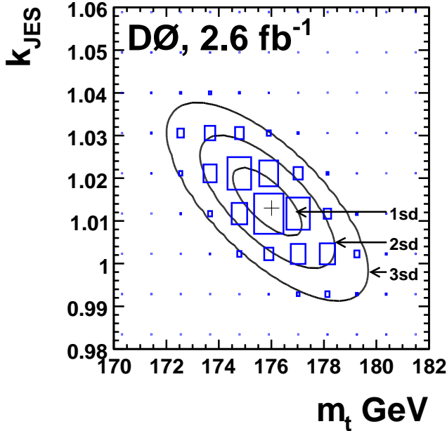
Figure 9. (color online) Fitted contours of equal probability for the two-dimensional likelihood L(\tilde{x}; m_t, k_{\text{JES}}) .
