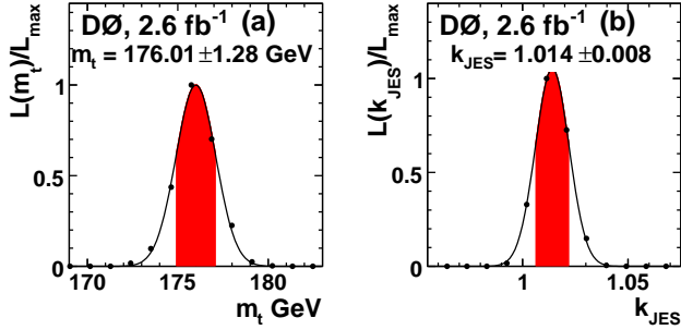
Figure 8. Calibrated projections of the data likelihoods onto the (a) m_t and (b) k_{\text{JES}} axes with 68% confidence level regions indicated by the shaded areas. The values of m_t and k_{\text{JES}} shown in the figures are after applying all the corrections described in Sec. VII and Sec. VIII.
