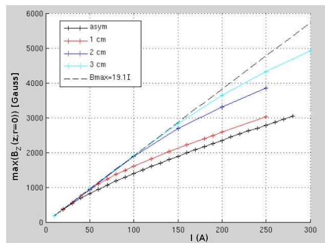
Figure 2: on-axis maximal longitudinal magnetic field component (from POISSON simulation of the “B3” solenoid) function of its current. The black dashed line is the linear approximation for low I values [ B_{max}(\text{Gauss}) = 19.1 I (\text{A}) ]. The black curve “asym” is the curve of the POISSON “B3” solenoid simulation. The red (resp. blue, cyan) curve is obtained with POISSON from a symmetric frame with 10 mm (resp. 20 mm, 30 mm) thick.
