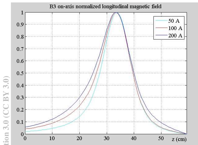
Figure 3: “B3” solenoid normalized on-axis longitudinal magnetic field component for different alimentation current ( I=50, 100 and 200 A).
