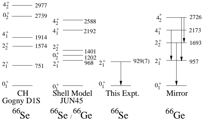
Figure 3: Experimental low-lying spectroscopy of ^{66}\text{Se} deduced from this work, compared to shell-model predictions with the JUN45 interaction [9] restricted to the pf_{5/2}g_{9/2} valence space and to CH calculations with the Gogny D1S interaction. Experimental low-lying levels for ^{66}\text{Ge} are from [35]. Energies are given in keV. For clarity, only the 2 first 0^+ , 2^+ and 4^+ , when possible, are shown.
