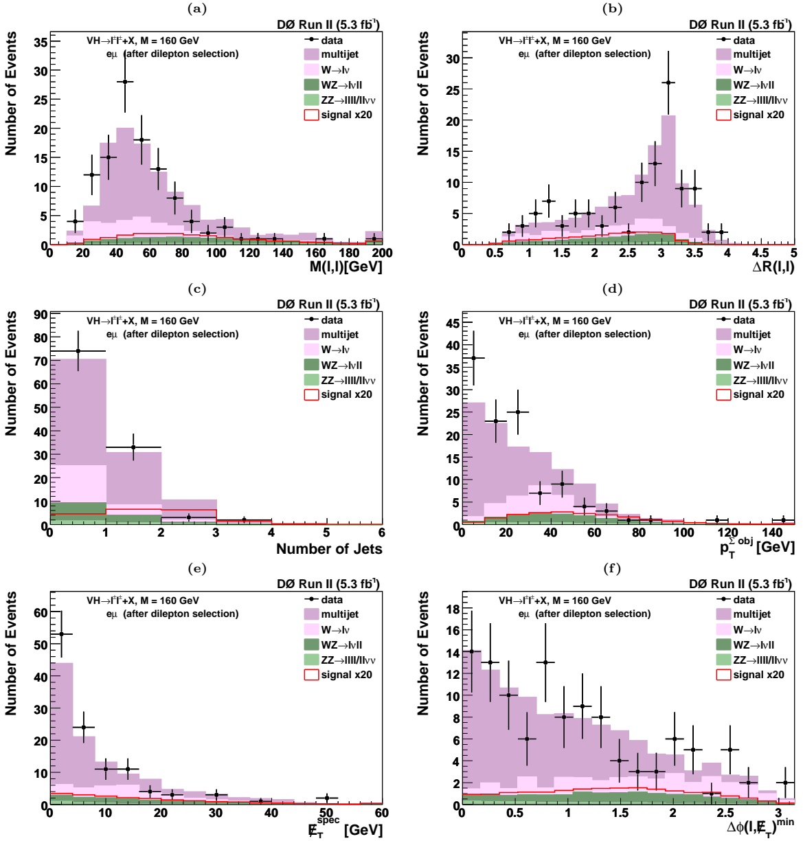
FIG. 3: (Color online) The distribution of (a) M(\ell, \ell) , (b) \Delta R(\ell, \ell) , (c) N_{\text{jet}} , (d) p_T^{\Sigma \text{obj}} , (e) E_T^{\text{spec}} , (f) \Delta\phi(\ell, \cancel{E}_T)^{\min} , for the e\mu channel comparing data and predicted backgrounds as well as the Higgs boson signal ( M_H = 160 GeV) expectation after the kinematic selection of like charge dilepton events. Due to the absence of charge flip background in e\mu channel, the sample after kinematic selection is dominated by multijet and W +jet backgrounds.
