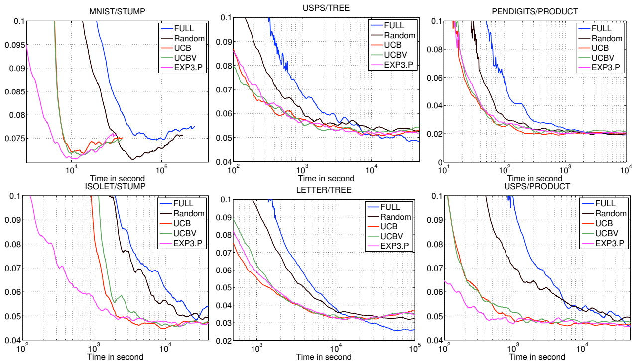
Figure 4. Smoothed test errors \bar{R}^{(T)} vs. total computational time.
