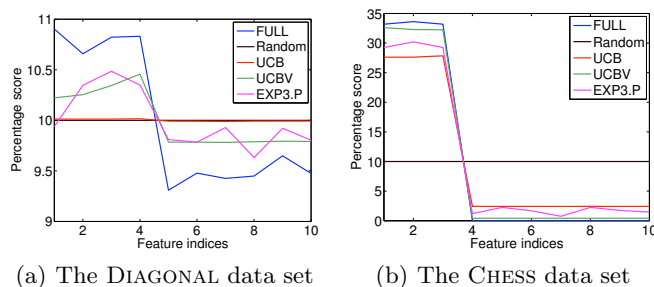
Figure 3. The percentage score of the iterations when a certain feature was selected on (a) \text{DIAGONAL}(10, 4, 0.1) and (b) \text{CHESS}(10, 3, 3) by the different algorithms.
