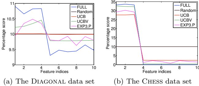
Figure 3. The percentage score of the iterations when a certain feature was selected on (a) \text{DIAGONAL}(10, 4, 0.1) and (b) \text{CHESS}(10, 3, 3) by the different algorithms.
