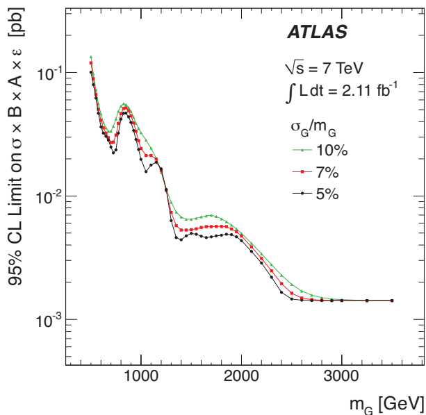
FIG. 2. The 95% CL upper limits on \sigma \times B \times A \times \epsilon for a hypothetical signal with Gaussian m_{\gamma j} distribution decaying to a photon and a jet as a function of the signal mass, m_G , for three values of the relative Gaussian width \sigma_G/m_G and taking into account systematic uncertainties.
