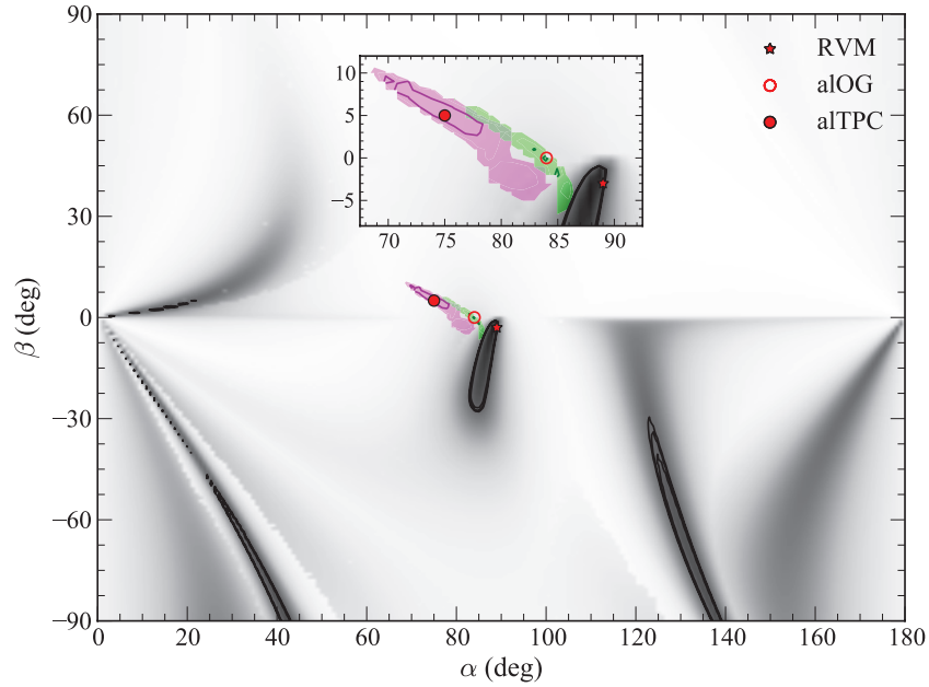
Figure 8. Plot of the impact angle \beta = \zeta - \alpha , vs. the magnetic inclination angle \alpha for PSR B1937+21. The \chi^2 map of the RVM fit of radio polarization data for PSR B1937+21 is shown in gray scale, with contour levels at 1\sigma , 2\sigma , and 3\sigma in black. Magenta and green shaded regions indicate the 3\sigma contour levels of the simultaneous radio and gamma-ray light curve modeling under the aTPC and aLOG geometries, while the solid lines show the 1\sigma contour levels. The symbols indicate the best pulsar orientation angles obtained from the RVM, aTPC, and aLOG fits.
