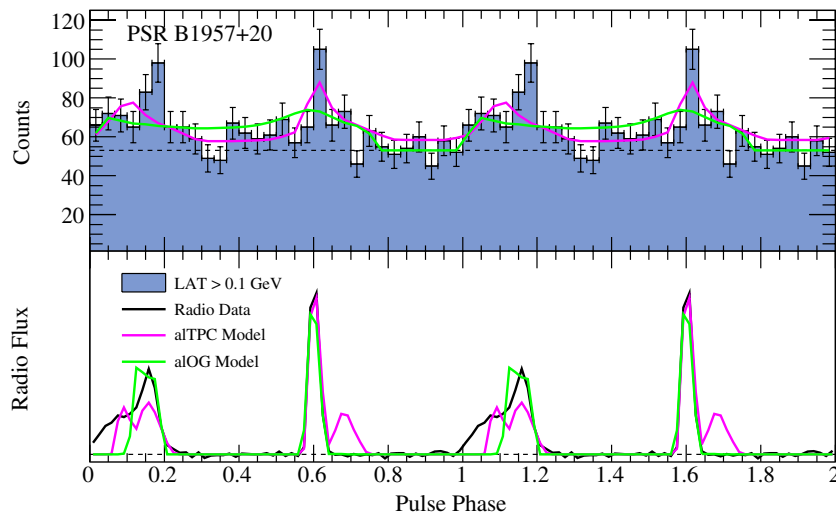
Figure 7. Same as Figure 6, for PSR B1957+20. The bottom panel shows the Westerbork 0.35 GHz radio profile. (A color version of this figure is available in the online journal.)
