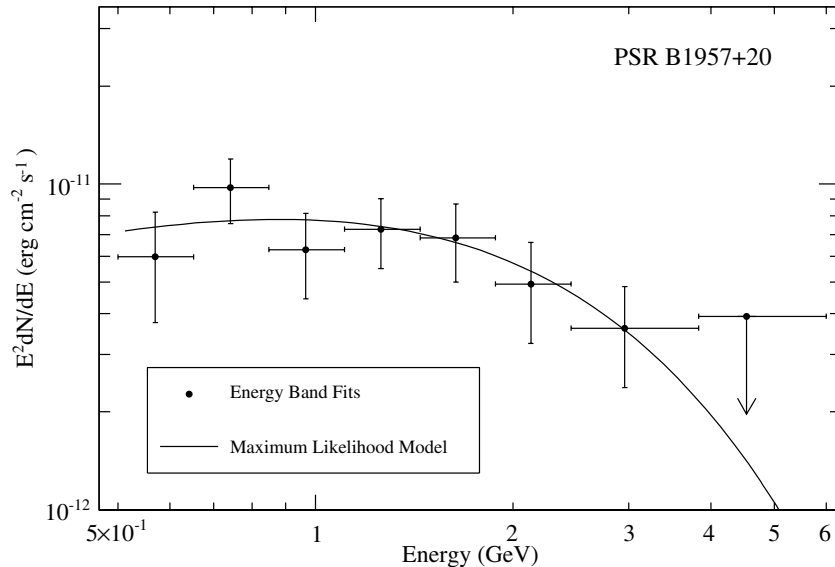
Figure 2. Same as Figure 1 for PSR B1957+20.
