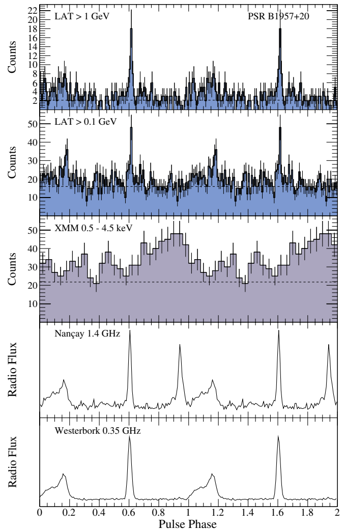
Figure 5. Same as Figure 4, for PSR B1957+20. The two bottom panels show radio profiles recorded at the Westerbork and Nançay radio telescopes at 0.35 and 1.4 GHz. The middle panel shows an X-ray profile obtained from an analysis of XMM-Newton data between 0.5 and 4.5 keV, with 25 bins per rotation. The background level in this panel was extracted from a similar neighboring region, free from X-ray sources. The two top panels show 100 bin gamma-ray light curves recorded with the LAT above 0.1 GeV and 1 GeV.
