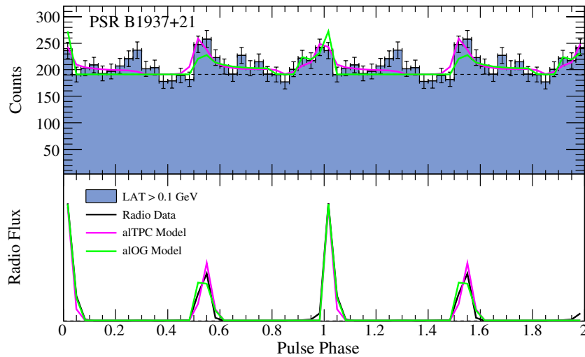
Figure 6. Top: gamma-ray data and modeled light curves for PSR B1937+21 with 30 bins per rotation. Bottom: Nançay 1.4 GHz radio profile and modeled light curves. See Table 3 for the best-fit parameters.
