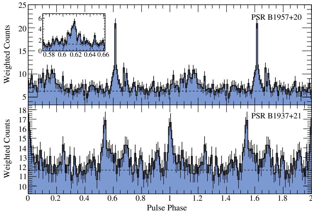
Figure 3. Gamma-ray light curves of PSRs B1937+21 (bottom panel) and B1957+20 (top panel) for events recorded by the Fermi LAT within 5^\circ from the pulsars, and with energies above 0.1 GeV. These profiles were built by weighting each event by its probability to have been emitted by the pulsars, where the probabilities have been obtained from the spectral analysis of the two MSPs (see Section 3.2.1 for more details). Two rotations are shown for clarity, and the light curves have 100 bins per rotation. The inset shows the profile of PSR B1957+20 in the 0.57–0.66 phase range, with 500 bins per rotation or \sim 3 \mu\text{s} per bin. (A color version of this figure is available in the online journal.)
