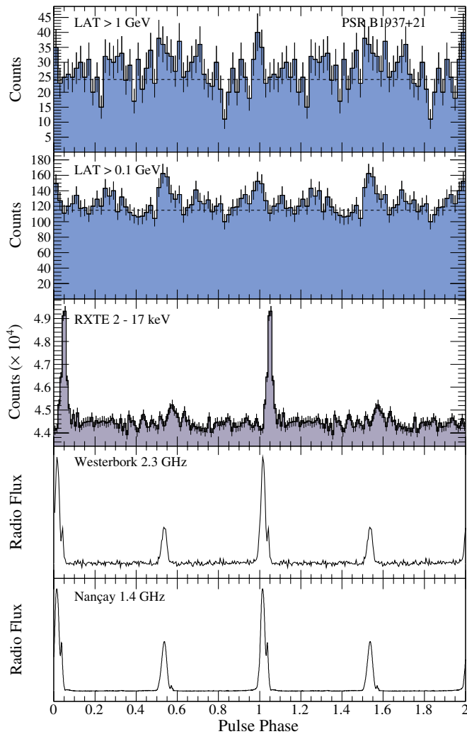
Figure 4. Multi-wavelength phase histograms of PSR B1937+21. The two bottom panels show radio profiles recorded at the Nançay and Westerbork radio telescopes at 1.4 and 2.3 GHz. The middle panel shows an X-ray light curve recorded with RXTE between 2 and 17 keV, with 100 bins per rotation. The two top panels show 50 bin gamma-ray light curves recorded with the LAT above 0.1 GeV and 1 GeV. Horizontal dashed lines indicate gamma-ray background levels (see Section 3.2.2 for details on the determination of these background levels).
