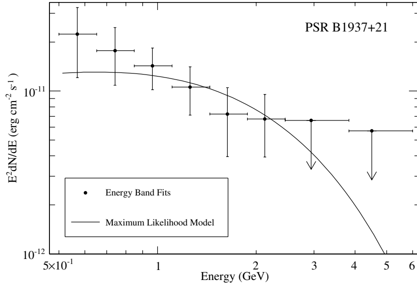
Figure 1. Phase-averaged gamma-ray energy spectrum for PSR B1937+21, above 0.5 GeV. The black line shows the best-fit model from fitting all the gamma-ray data above 0.5 GeV with the simple exponentially cutoff power-law functional form given in Equation (1). Data points are derived from likelihood fits of individual energy bands where the pulsar is modeled with a simple power-law form. A 95% confidence level upper limit was calculated for any energy band in which the pulsar was not detected above the background with a significance of at least 2\sigma .
