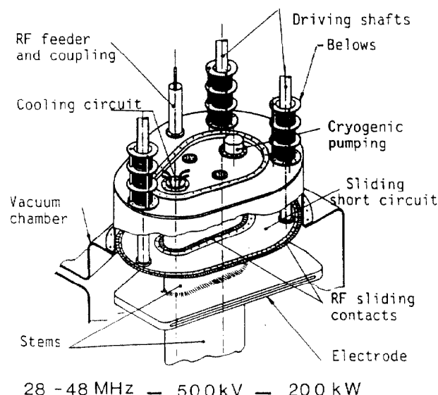
Figure 8 : Sketch of an accelerating cavity
