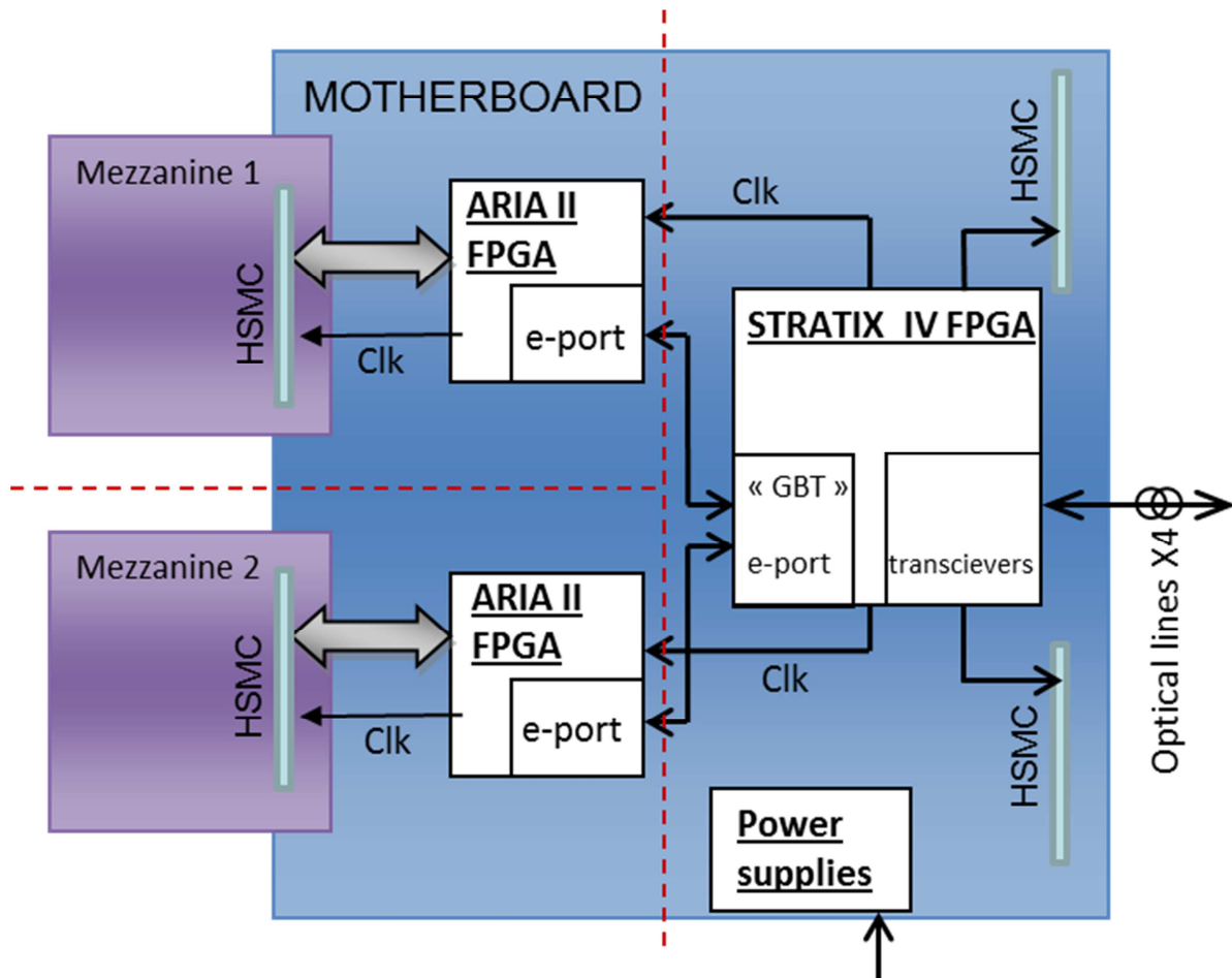
Emulation board architecture.
