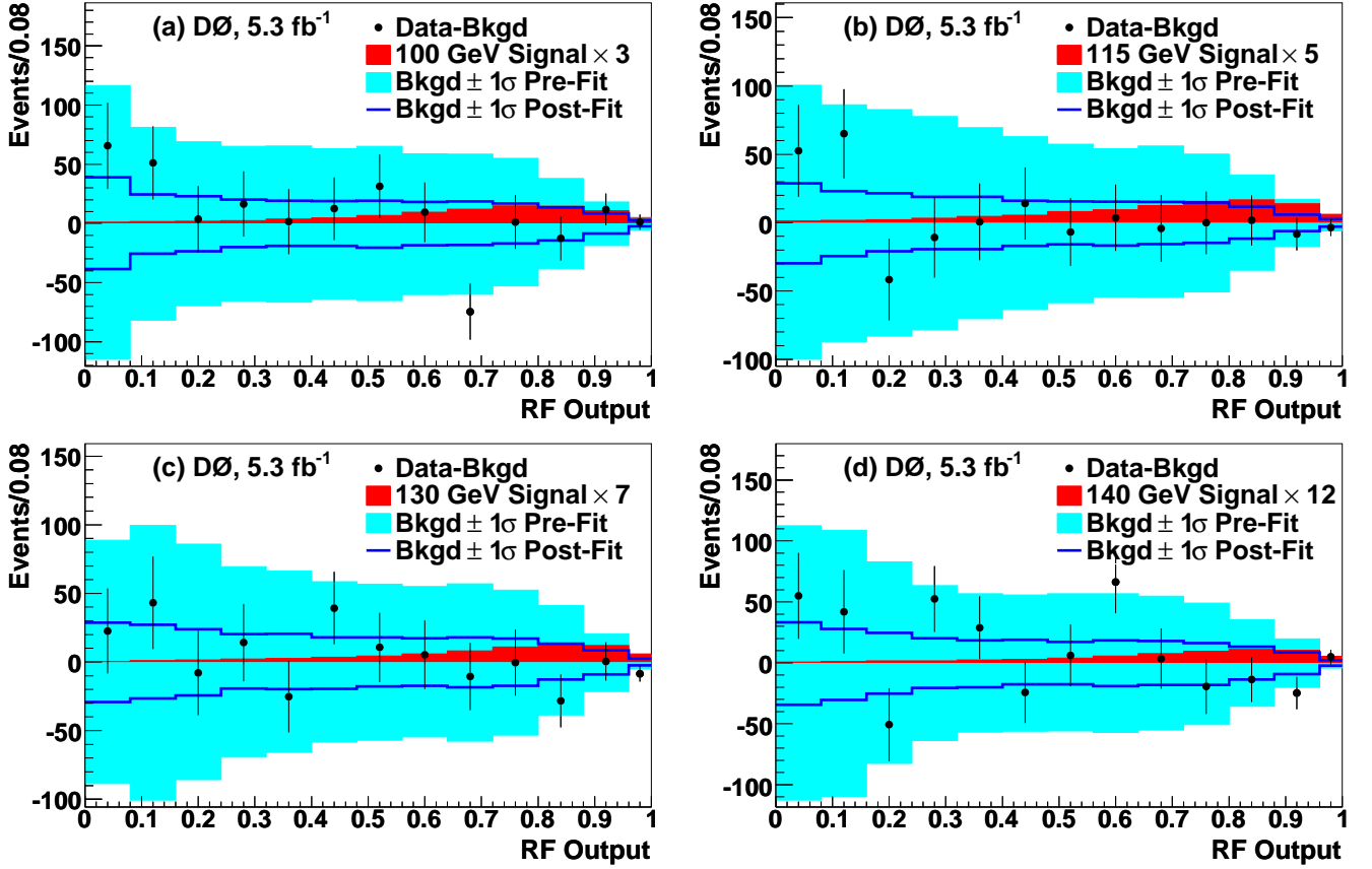
FIG. 13: [color online] The RF discriminant output distribution minus the total background expectation for (a) M_H = 100 GeV, (b) M_H = 115 GeV, (c) M_H = 130 GeV, and (d) M_H = 140 GeV. The pre-fit uncertainties are shown by the shaded bands and the post-fit uncertainties are represented by the solid lines. The signal expectation is shown scaled to the obtained observed upper limit at each test mass point.
