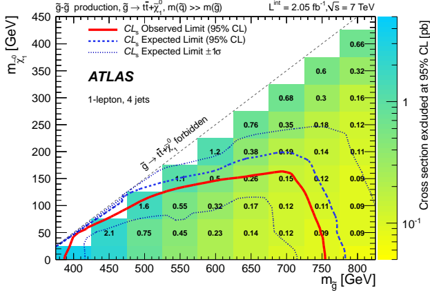
FIG. 9: The observed and expected 95% CL exclusion limits in the (m_{\tilde{g}}, m_{\tilde{\chi}_1^0}) plane ( Gtt ) using the best expected limit between SR1-D and SR1-E for each signal point.
