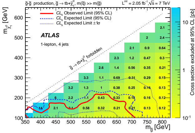
FIG. 10: The observed and expected 95% CL exclusion limits in the (m_{\tilde{g}}, m_{\tilde{\chi}_1^0}) plane ( Gtb models) using the best expected limit between SR1-D and SR1-E for each signal point.
