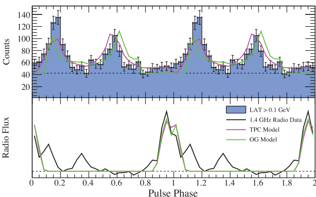
Figure 3. Data and best-fitting light curves using the gamma-ray data described in Section 3.1 (top) and the 1.4 GHz radio profile (bottom). Models corresponding to the TPC fit are shown as dot-dashed lines (solid pink lines online) and for the OG fit as dashed lines (solid green lines online).
