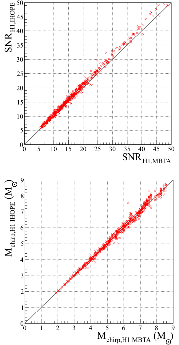
Fig. 11. Comparison of chirp mass and SNR between MBTA and CBC offline analysis pipeline.
