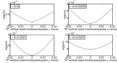
Figure 2: Vertical beam size change function of vertical waist knob S, for different settings of the coupling knob K.
