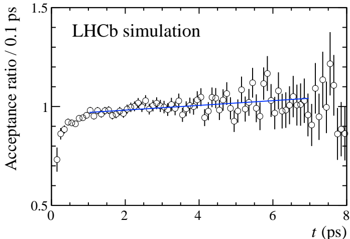
Figure 2: Ratio of decay time acceptances between \bar{B}_s^0 \rightarrow J/\psi f_0(980) and \bar{B}^0 \rightarrow J/\psi \bar{K}^{*0} decays obtained from simulation. The solid (blue) line shows the result of a linear fit.
