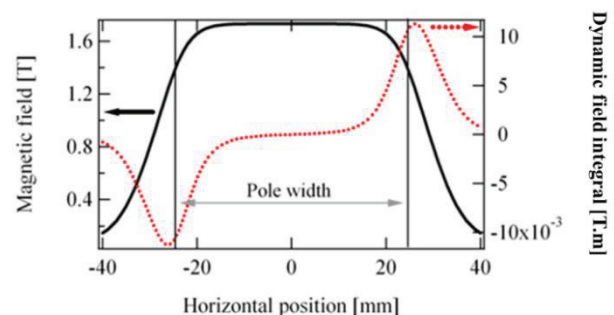
Figure 2: Transverse variation of the field (—) at minimum gap and Dynamic Field Integral (...).
