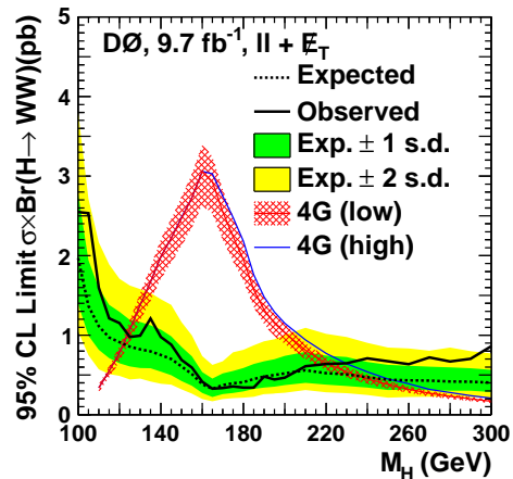
FIG. 4: [color online] Excluded cross section \sigma(gg \rightarrow H) \times BR(H \rightarrow WW) in pb as a function of M_H using all channels. The red and blue lines correspond to the theoretical prediction for a sequential fourth generation assumption in the “low mass” and “high mass” scenarios, respectively (see main text). The hatched region corresponds to the PDF and scale uncertainties on the fourth generation “low mass” prediction [50]. The green and yellow shaded bands indicate \pm 1 and \pm 2 s.d. uncertainties of the background-only hypothesis, respectively.
