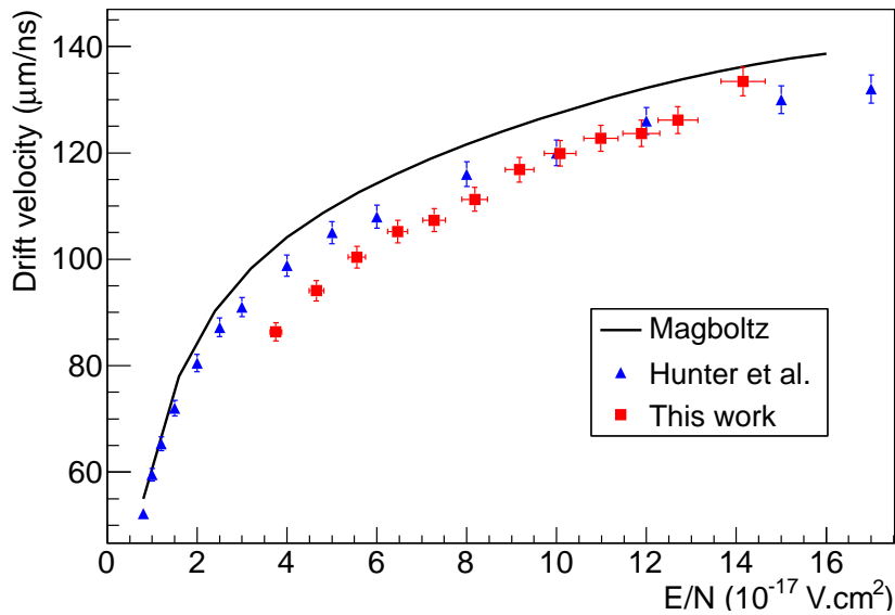
Figure 10. Electron drift velocity measurement v_d ( \mu\text{m/ns} ) in a pure CF_4 gas at 50 mbar as a function of E/N ( 10^{-17} \text{Vcm}^2 ), for an amplification field E_a = 14.5 kV/cm. The data (red squares) have been obtained with the likelihood analysis strategy. We also present the Magboltz simulation (black line) and previous experimental data (blue triangle) [38].
