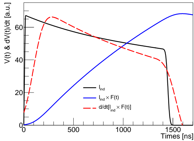
Figure 5. Theoretical signal V_{th}(t) (blue curve) obtained from the convolution of the current induced on the grid I_{ind}(t) (black curve) and the transfer function of the charge preamplifier F(t) . The dashed red curve is the time derivative V'_{th}(t) of the signal V_{th}(t) .
